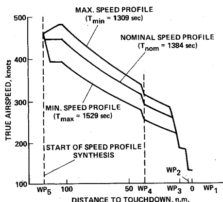
Fig. 1 Controlled time of arrival speed profiles.
